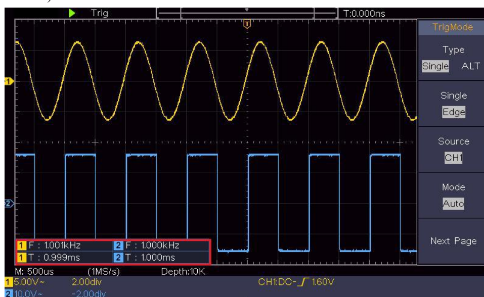
Figure 4- 12 Automatic measurement
