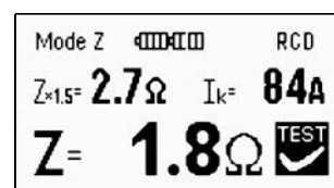
Figure 3.22: Impedance Downstream from an RCCB (detailed)
