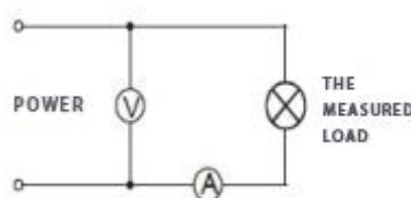
Fig. 5 Measurement Principle
