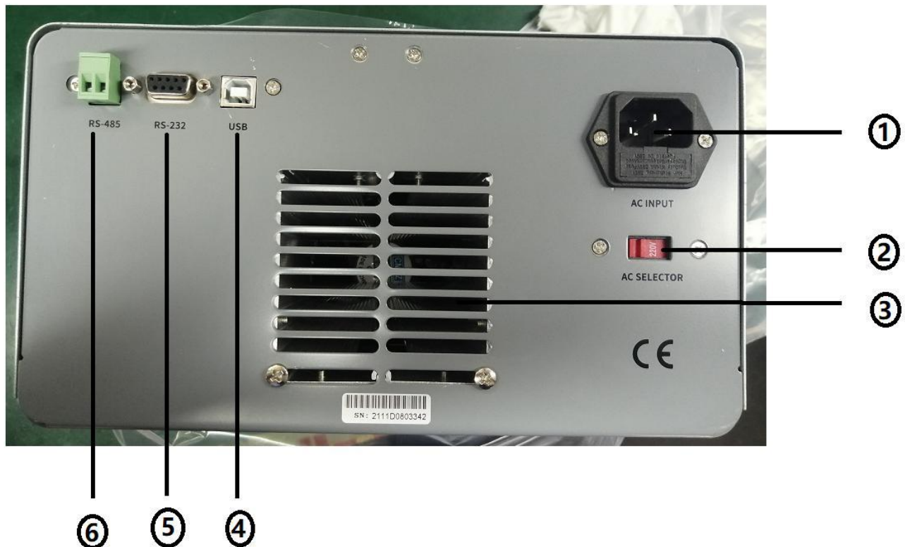
Figure 3.2 Rear panel of MPS-H-3 series DC power supply
