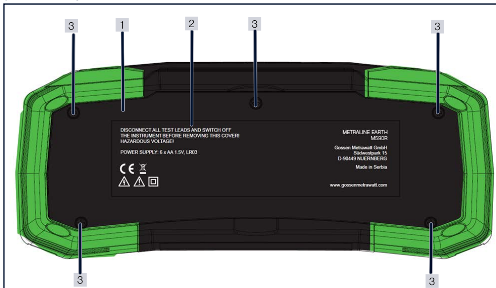
Fig. 2: Back of Instrument
