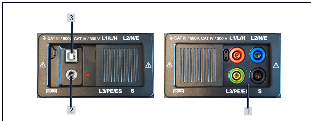
Fig. 3: Top of Instrument
