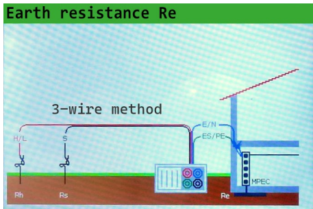
Fig. 7: Earth Resistance Measurement R_e , Wiring and Results
