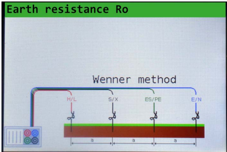
Fig. 8: Earth Resistance Measurement R_o , Wiring and Results
